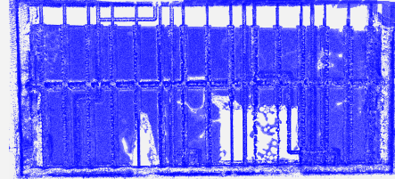
(Fig. 5.3) Plot of the centers of the gaussians comprising the wall. The two large holes near the base are result of geometry which is out-of-plane. (c.f. Fig 6.)
